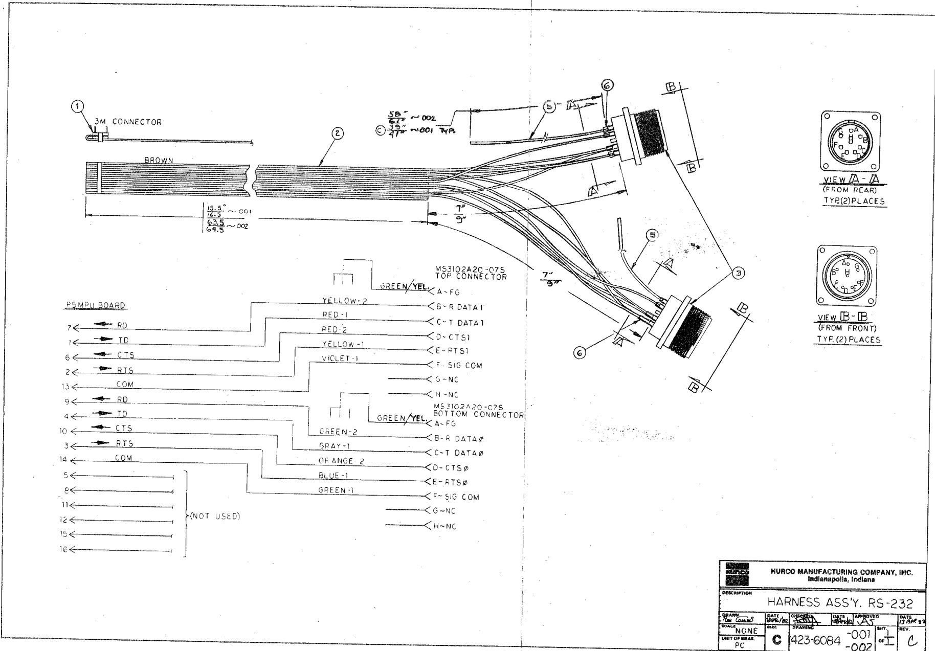
Figure 7-13 RS-232 Harness Assembly
