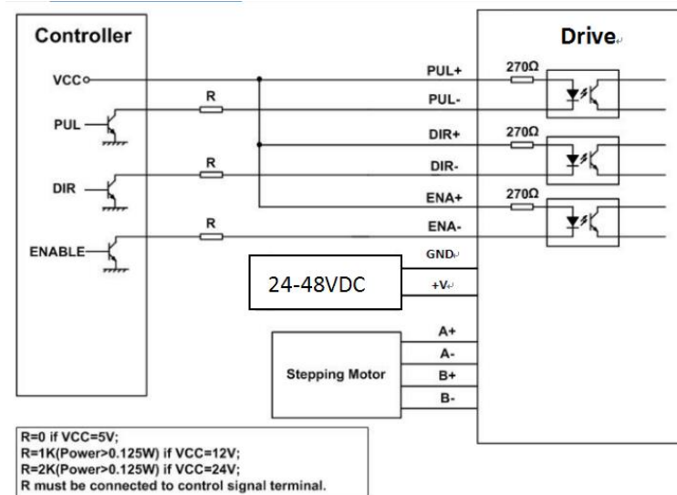
Figure 9: Typical connection
