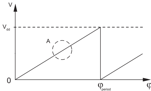
Fig. 5: Timing diagram for linear voltage output
